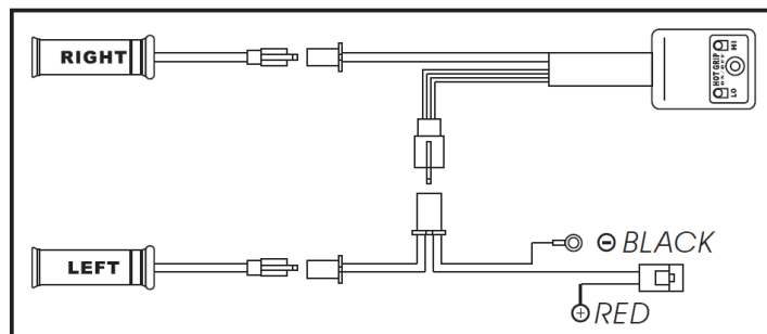
Diagram for how to connect wiring leads
